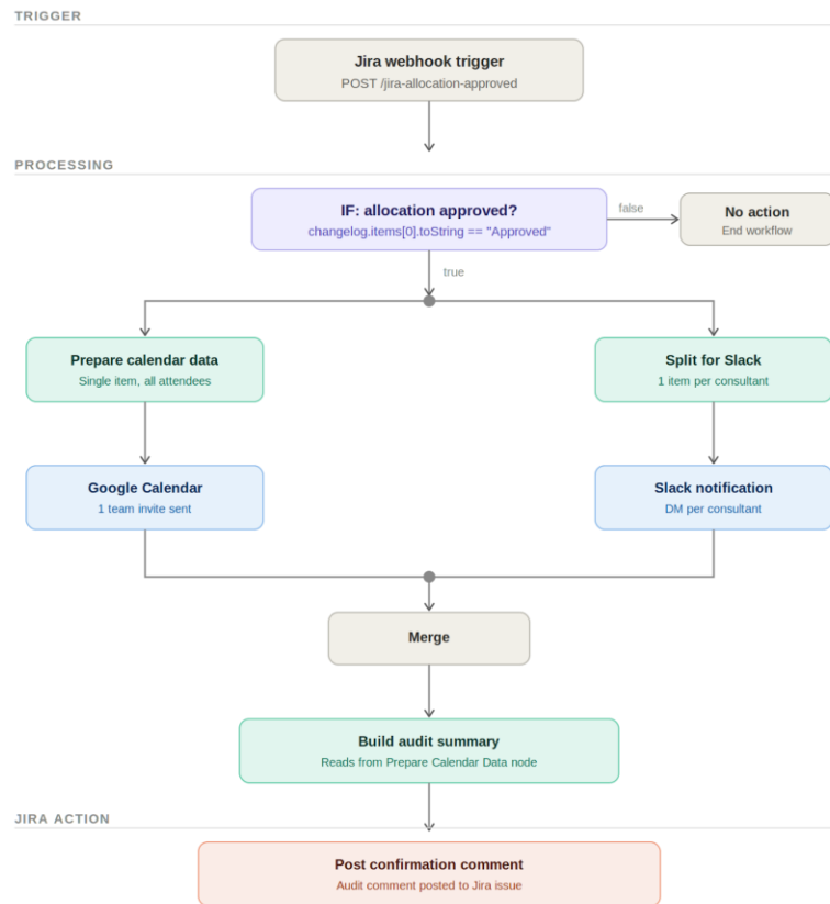
Figure 1 — SIL-15 n8n workflow: Trigger → Processing → Jira Action
